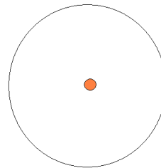
6. Photons are compressed to the limit
