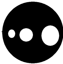
3. The penetration of the stream of photons to the emptiness
