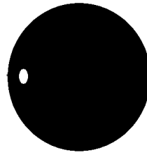
2. The penetration of a photon to the emptiness
