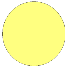
5. Photons are heated up to the limit
