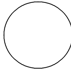
4. The emptiness is filled with photons
